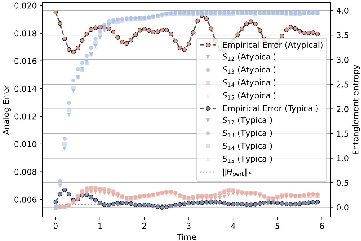
2D-lattice QIMF, one segment evolution with disorder & imperfections
